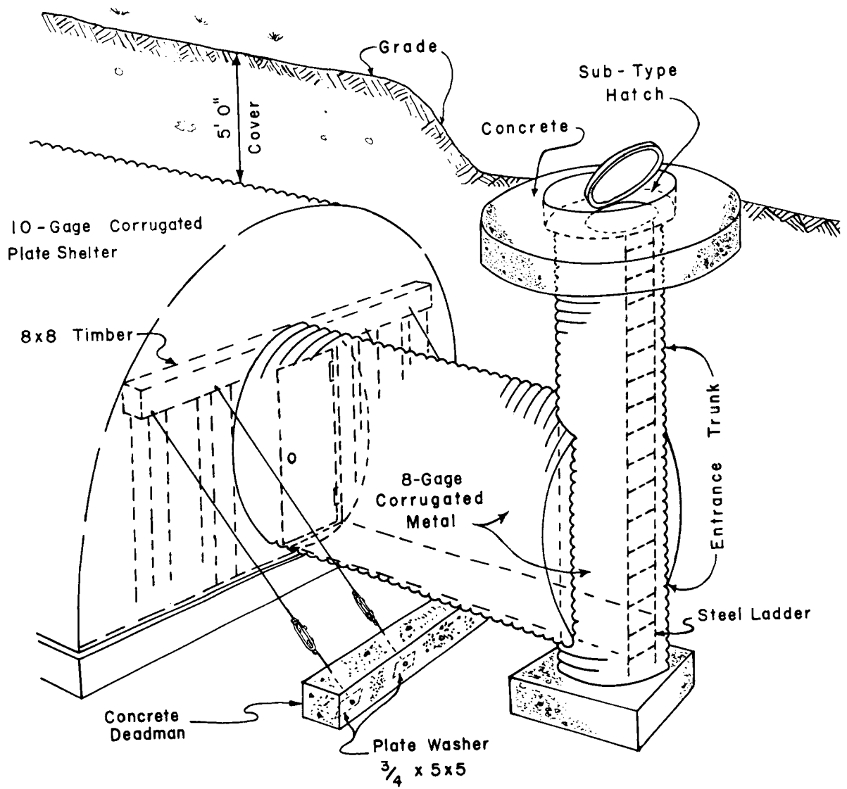
Fig. 8—Sketch of shelter entrance.
